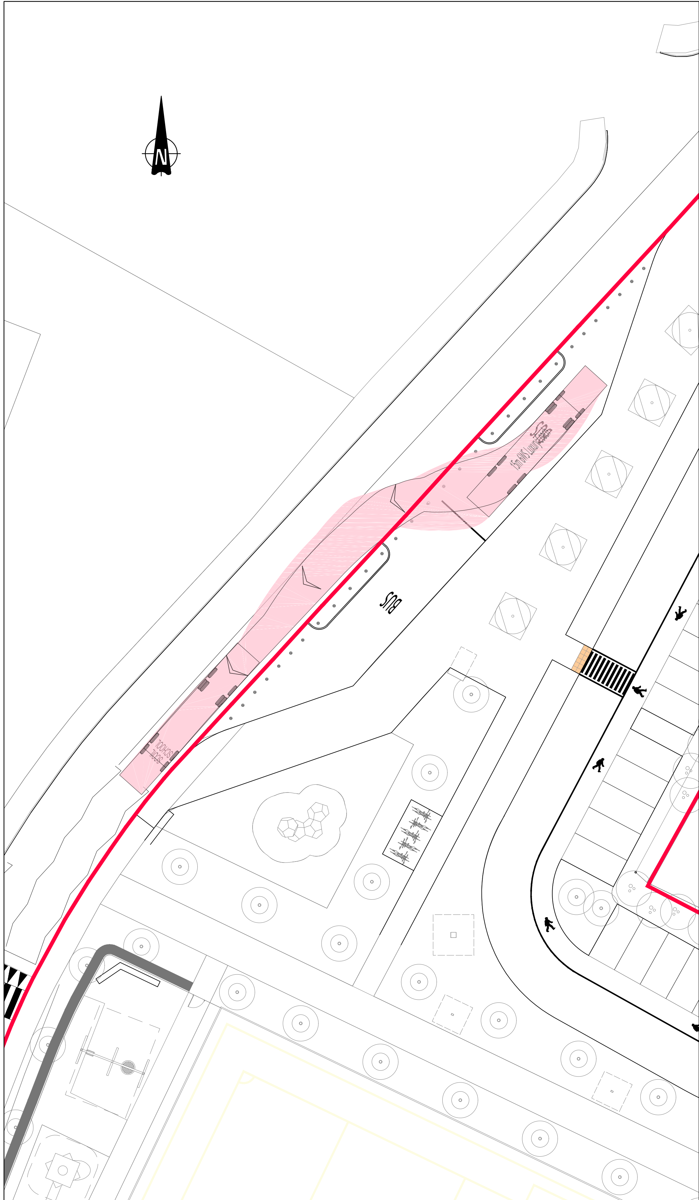
DETAIL 2 - DESIGN VEHICLE EXITING BY ALTERNATIVE EXIT SCALE 1:200
